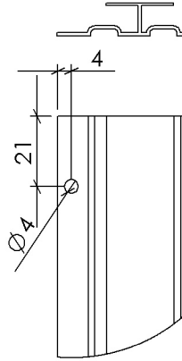
DETAIL B SCALE 1 : 2
